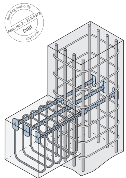
Corbel with HALFEN HSC Stud connector
