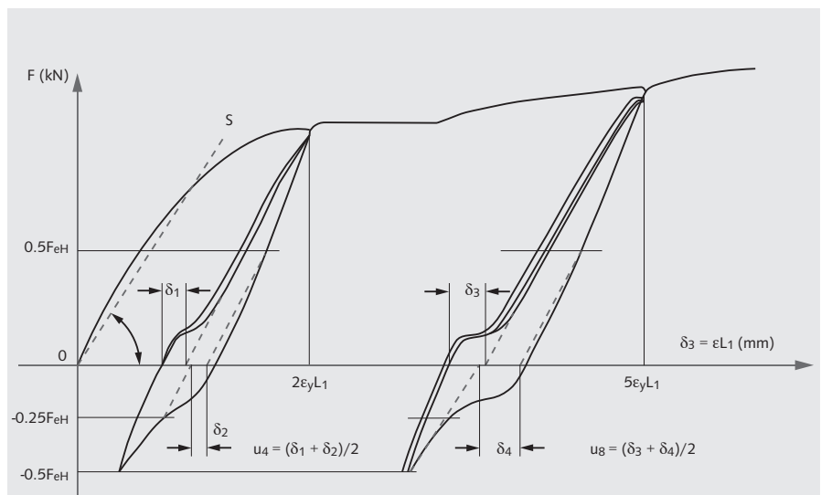
Diagram: Shows an experiment done in a series of test with HBS-05-Seismic under cyclic loading according to ISO 15835: In large earthquake after 8 cycles the residual elongation u_8 , between the strain of 5 \epsilon_y on the tension side and contraction of -0.5 f_y on the compression side, must not exceed 0.6 mm.
